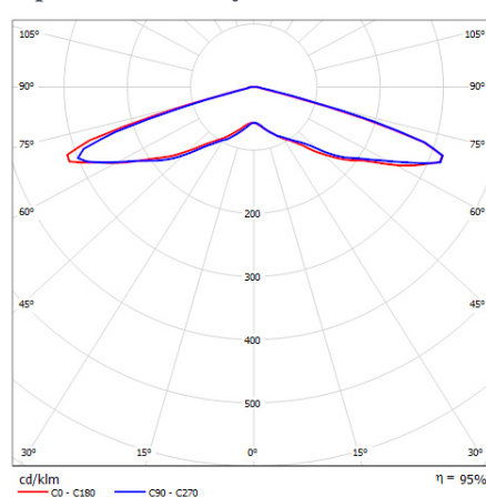
Optic B – roundsymmetric
