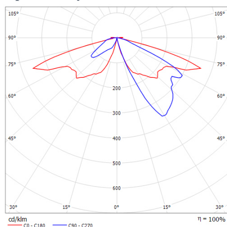
Optic A – asymmetric
